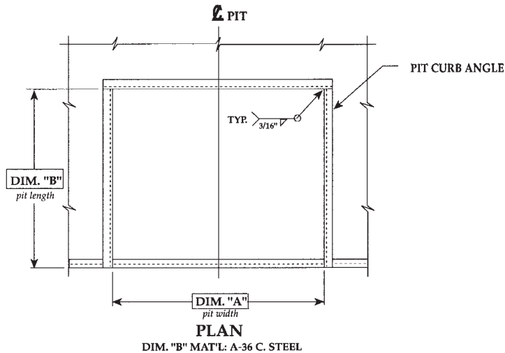
FIGURE B – PLAN VIEW
